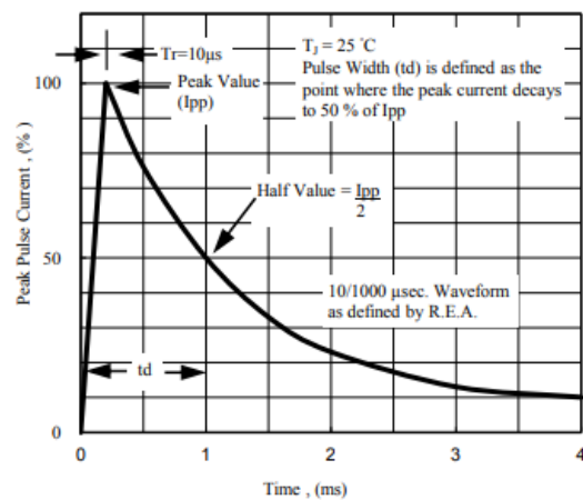
Figure 4- Pulse Waveform
