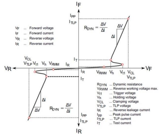
Figure 2- V-I Curve
