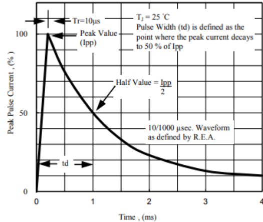
Figure 4- Pulse Waveform
