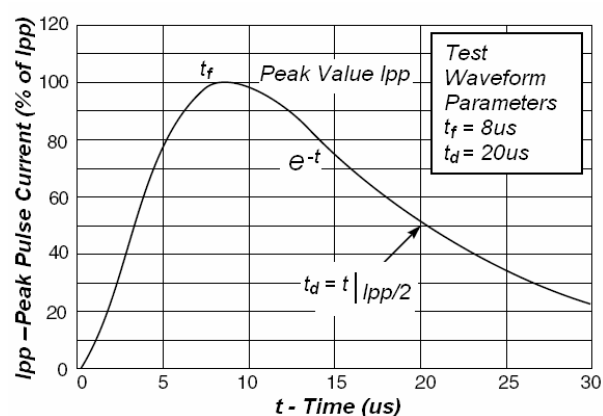
Figure 2- Pulse Waveform
