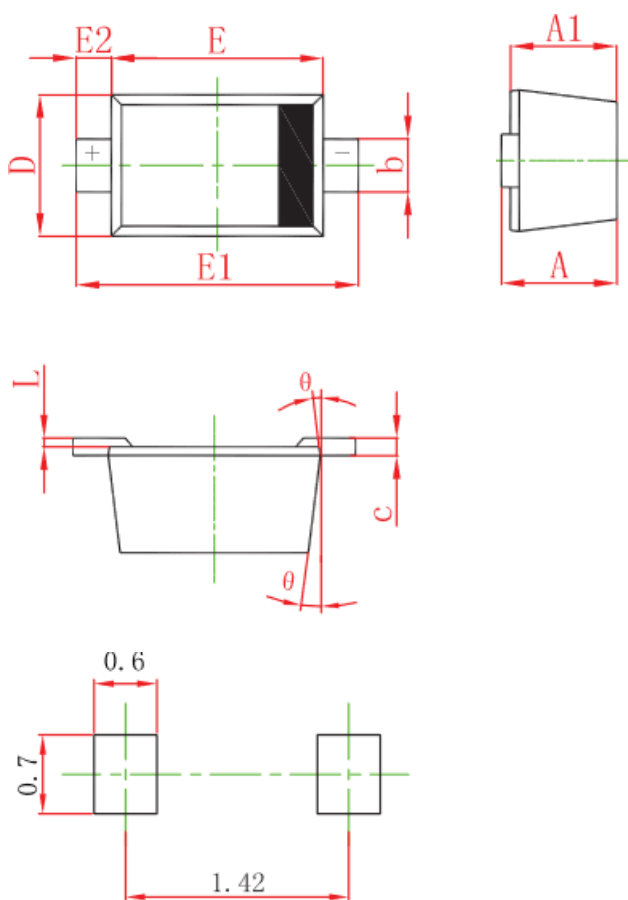
Pad Layout
