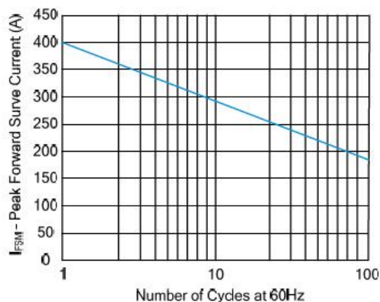
Figure 3- Maximum Non-Repetitive Forward Surge Current Uni-Directional Only
